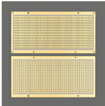
DPC ceramic circuit panels with fine metallized patterns
